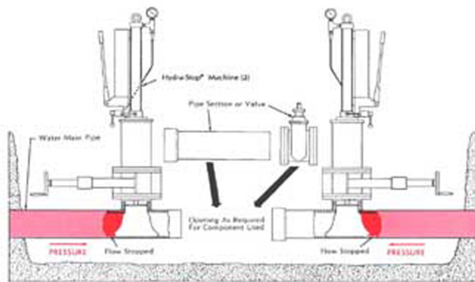
DOUBLE HYDRA-STOP® SYSTEM WITH WATER PRESSURE FROM TWO SIDES (LOOPED WATER CIRCUIT)
